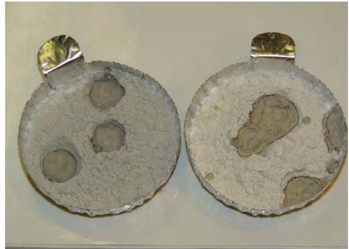
Wetted silica dust takes on the characteristics of mud, as shown in these samples. A dry environment should be maintained whenever possible to prevent the muddy dust from clogging filters.
